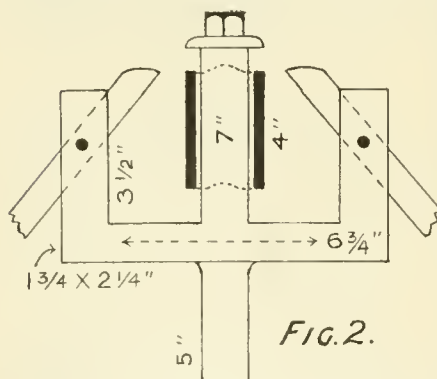
DOUBLE CUTTER FOR ROCKER ARMS.
